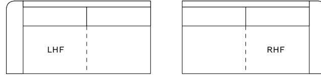
Manu 3P one arm W:1890 D:960 H:810 SH:440
