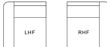
Manu one arm W:900 D:960 H:810 SH:440
